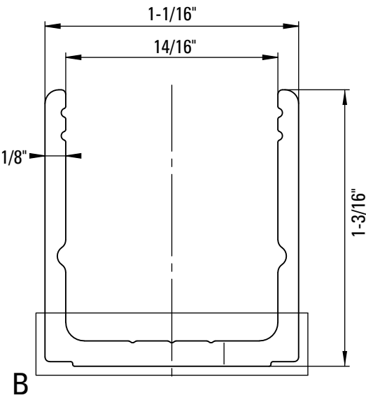
Profile: 1/2" - 9/16" Glass
